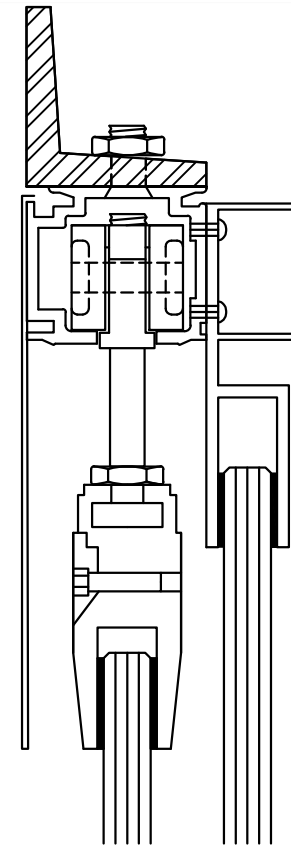
2 SIDELITE HEADER SECTION SCALE : 6"=1'-0"
