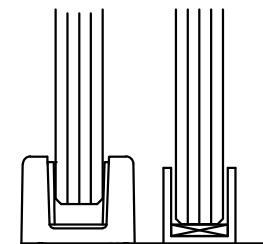
4 FLOOR GUIDE AND SIDELITE CHANNEL SECTION SCALE : 6"=1'-0"
